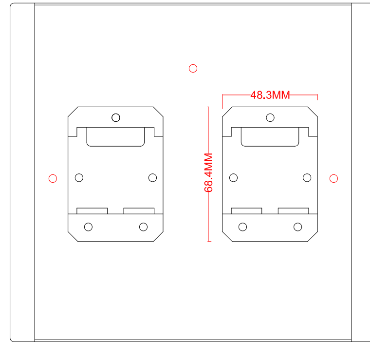
Bottom View with DIN Rail
